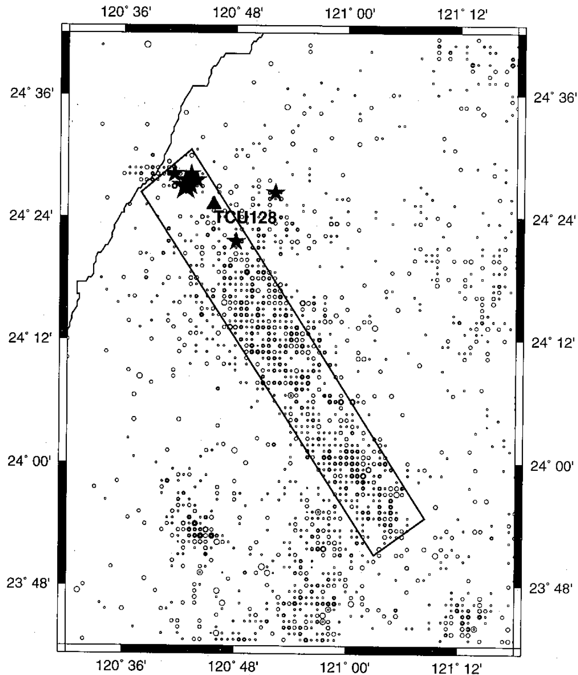
Figure 1. Seismicity in northwestern Taiwan. The box outlines the surface projection of the Sanyi-Tungshih-Puli seismic zone and hypothesized area of fault rupture for a M=7.25 earthquake. The stars indicate locations of events used to obtain empirical Green's functions, and TCU128 is the station location (NSY).
