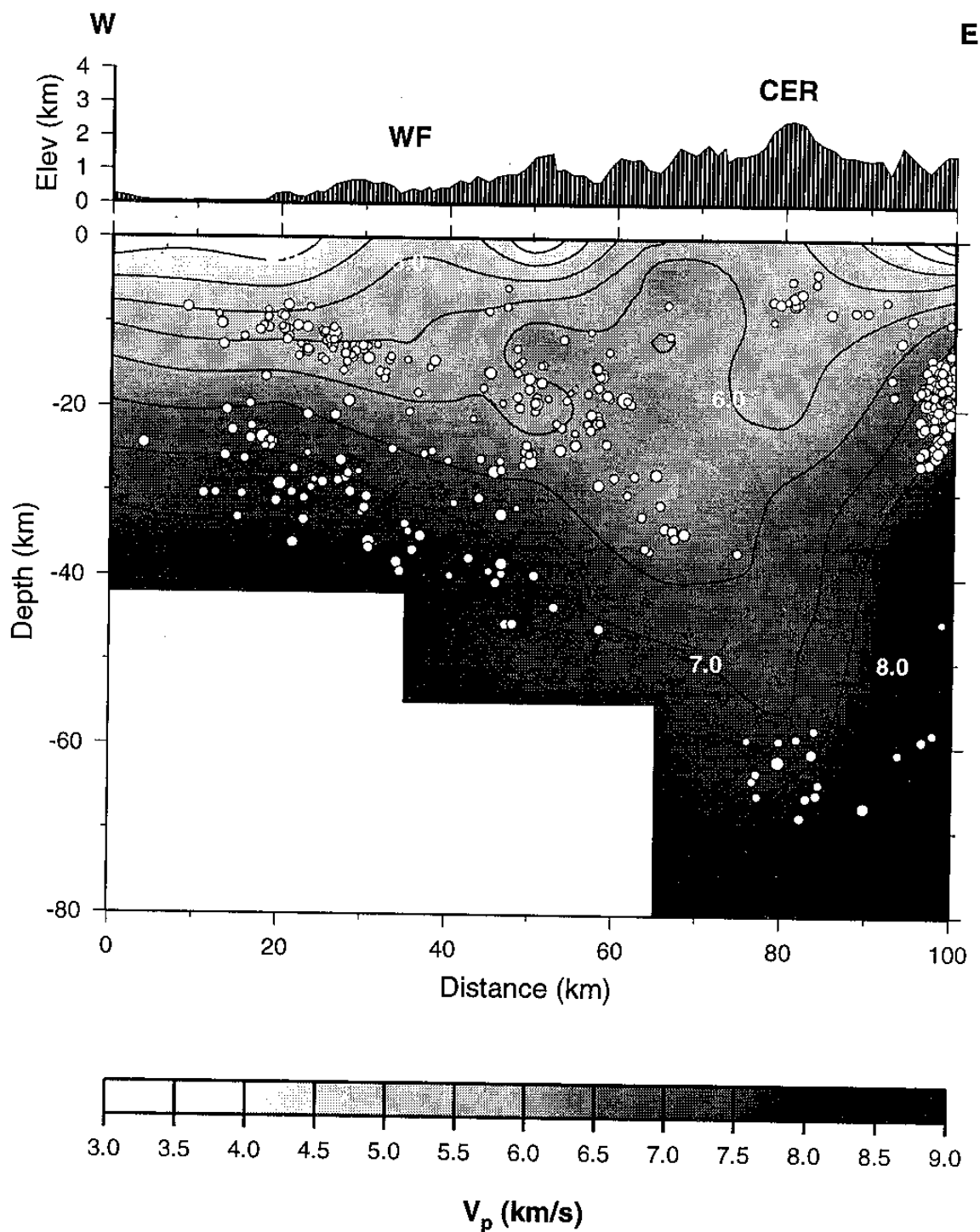
Figure 2. A cross section of seismicity across the Sanyi-Tungshih-Puli seismic zone (from Rau and Wu, 1995). The upper band of seismicity extends to about 20 km depth, and the lower band extends to about 60 km depth. Fault rupture is modeled for the upper band of seismicity.
